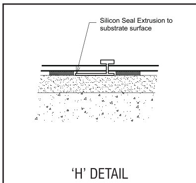
HAIRLINE JOINT
