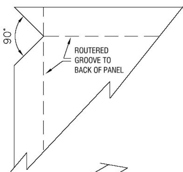
DETAIL OF CUT-OUT TO CORNER
