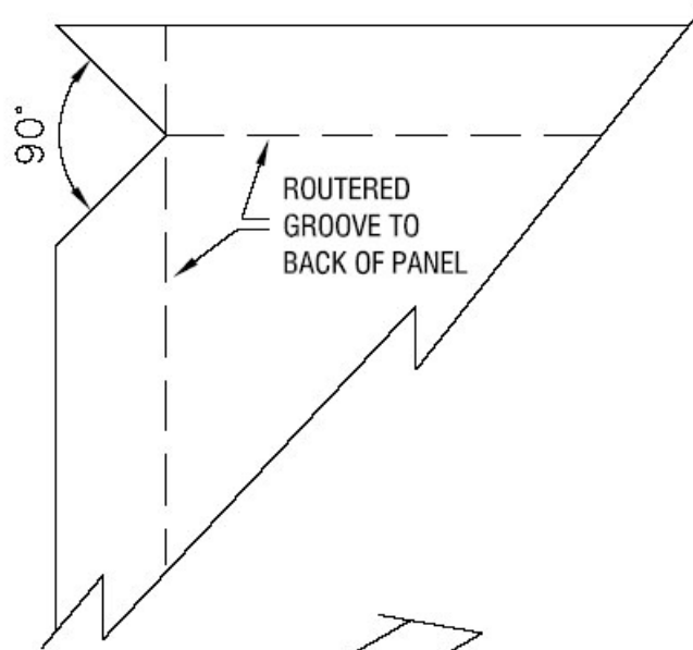
DETAIL OF CUT-OUT TO CORNER
